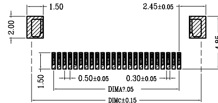
Suggested PCB Layout (Top View) (Tolerance: ±0.05)
