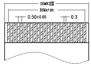
FFC Flexible Flat cable
