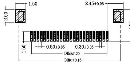
Suggested PCB Layout (Top View) (Tolerance: ±0.05)
