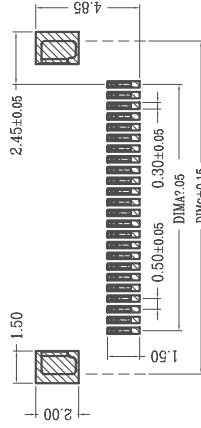
Suggested PCB Layout (Top View) (Tolerance: ±0.05)
